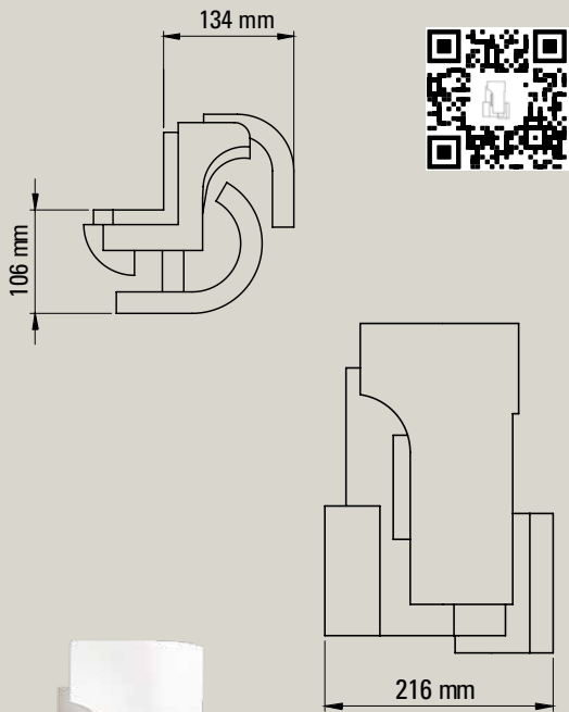
SOUL 5 WH-GOLD
