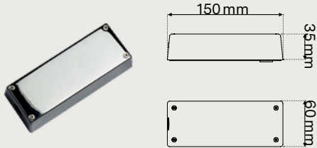
DRIVER BOX S Dimensions : 60 x 35 x 150 mm
