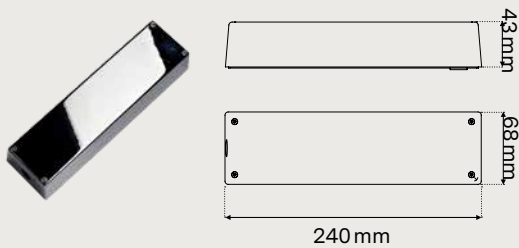
DRIVER BOX L Dimensions : 68 x 43 x 240 mm
